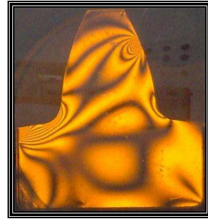
Fig. 21: Test No. 6-(15/28)-gear-monochromatic light
