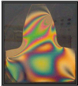
Fig. 26: Test No. 8-(18/22)-gear-white light
