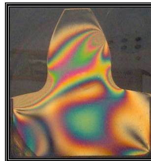
Fig. 24: Test No. 7-(18/22)-pinion-white light
