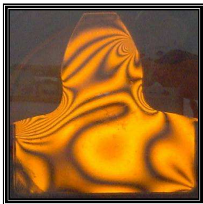
Fig. 11: Test No. 1 (15/18)-pinion-monochromatic light
