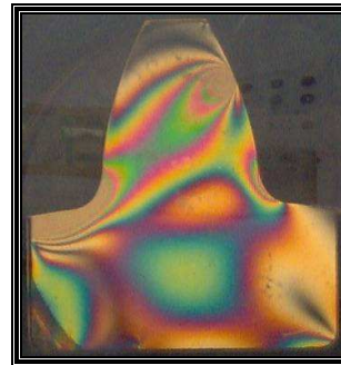
Fig. 22: Test No. 6-(15/28)-gear-white light
