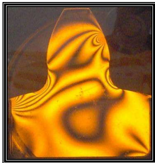
Fig. 19: Test No. 5-(15/28)-pinion-monochromatic light
